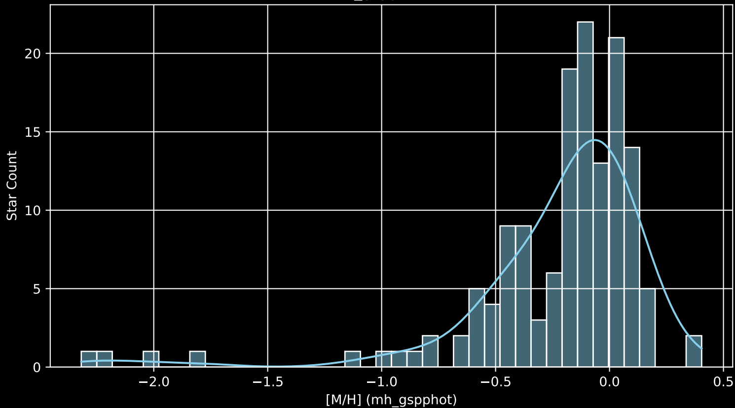
APOGEE DR17 Field: [340-12 [M/H] (mh_gspphot) (n= 144)
