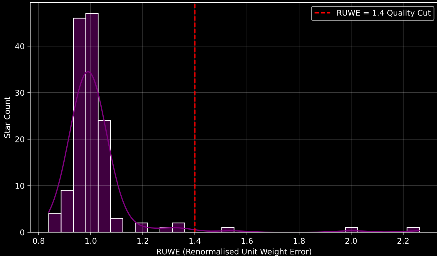
GAPOGEE DR17 Field [340-12] RUWE Distribution (n= 141)
