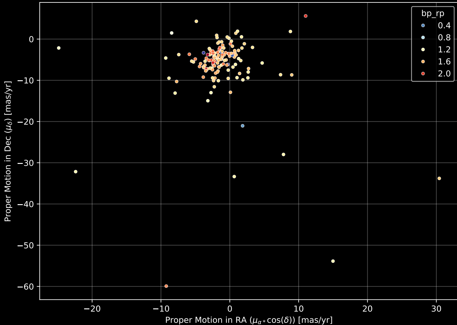
APOGEE DR17 Field: [340-12] Proper Motion Diagram (n= 144)
