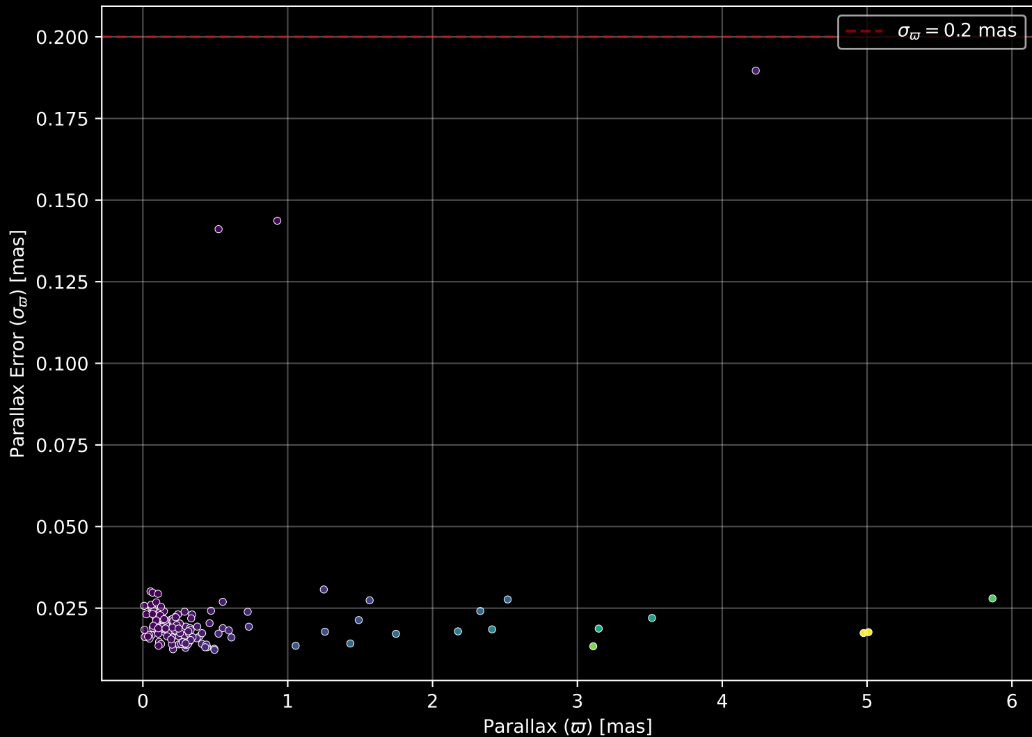
APOGEE DR17 Field: [340-12] Parallax Quality (n= 144)
